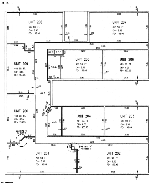
SECOND LEVEL INTERIOR WALLS 0.41" WIDE, OR AS NOTED EXTERIOR WALLS 1.20" WIDE, OR AS NOTED
