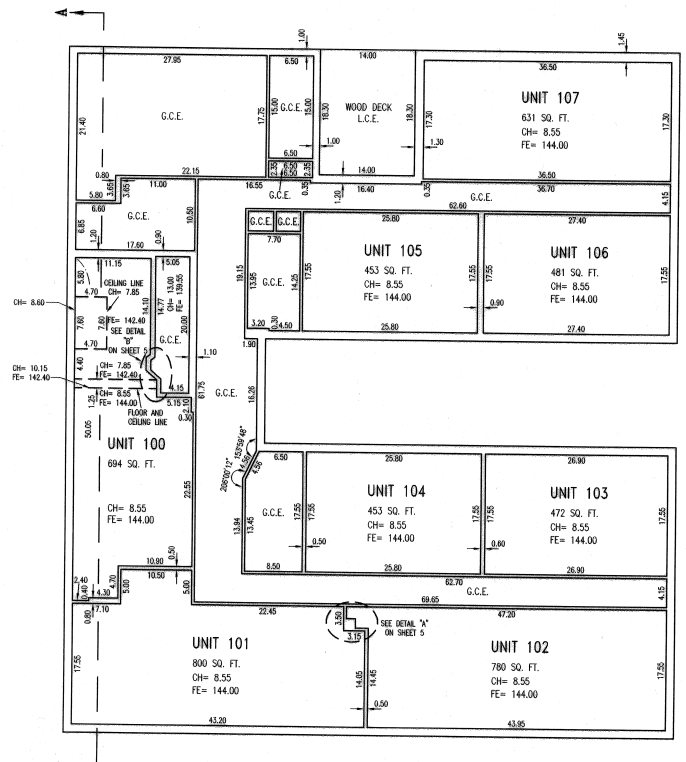
FIRST LEVEL INTERIOR WALLS 6.40" WIDE, OR AS NOTED EXTERIOR WALLS 1.20" WIDE, OR AS NOTED
